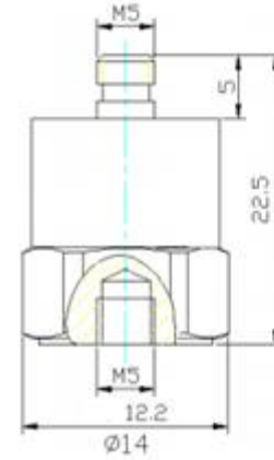
Schematic diagram
