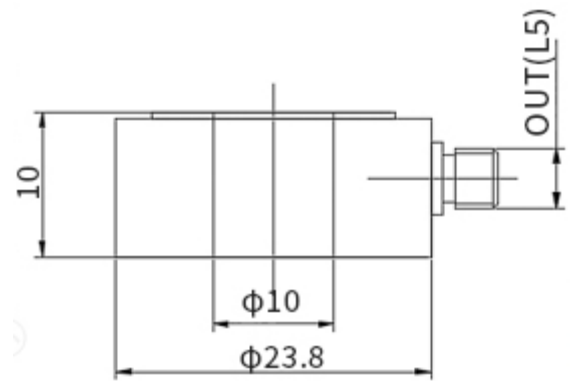
Schematic diagram
